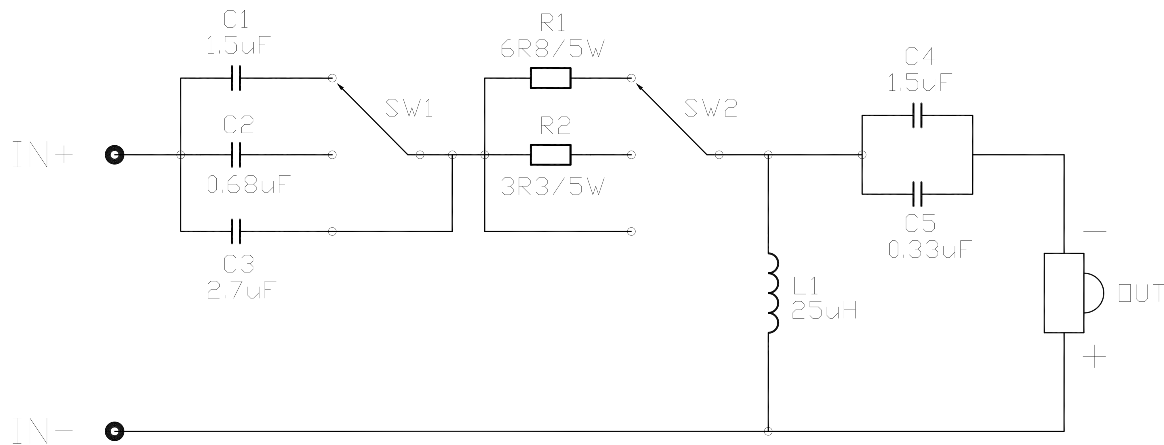
SCHEMATIC DIAGRAM
