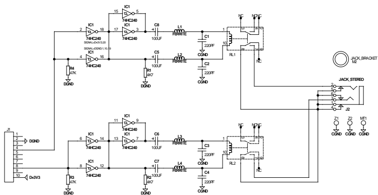
Manhattan Relayboard PCB 01
