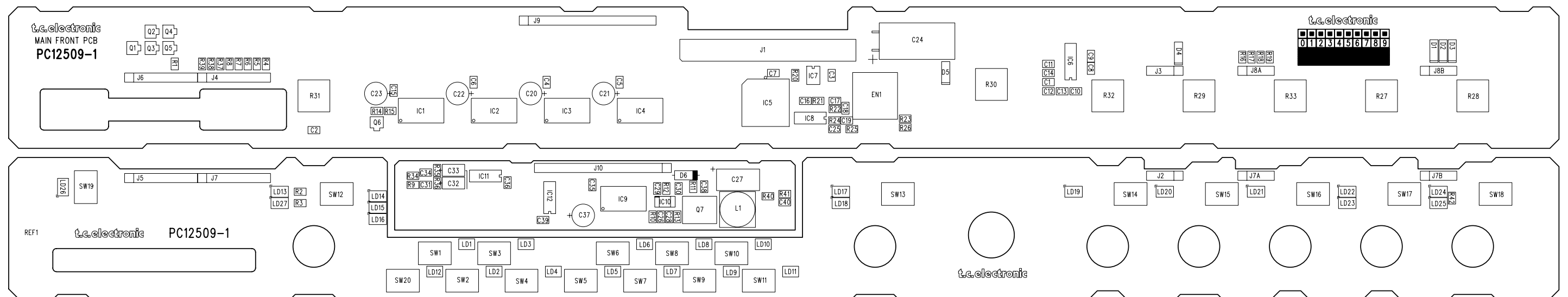
Layout Intonator Front PC12509-1
