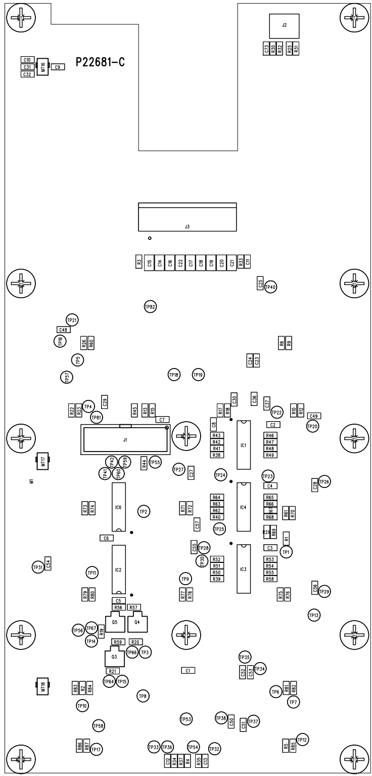
P22681 Lyr.1 Top Copper
