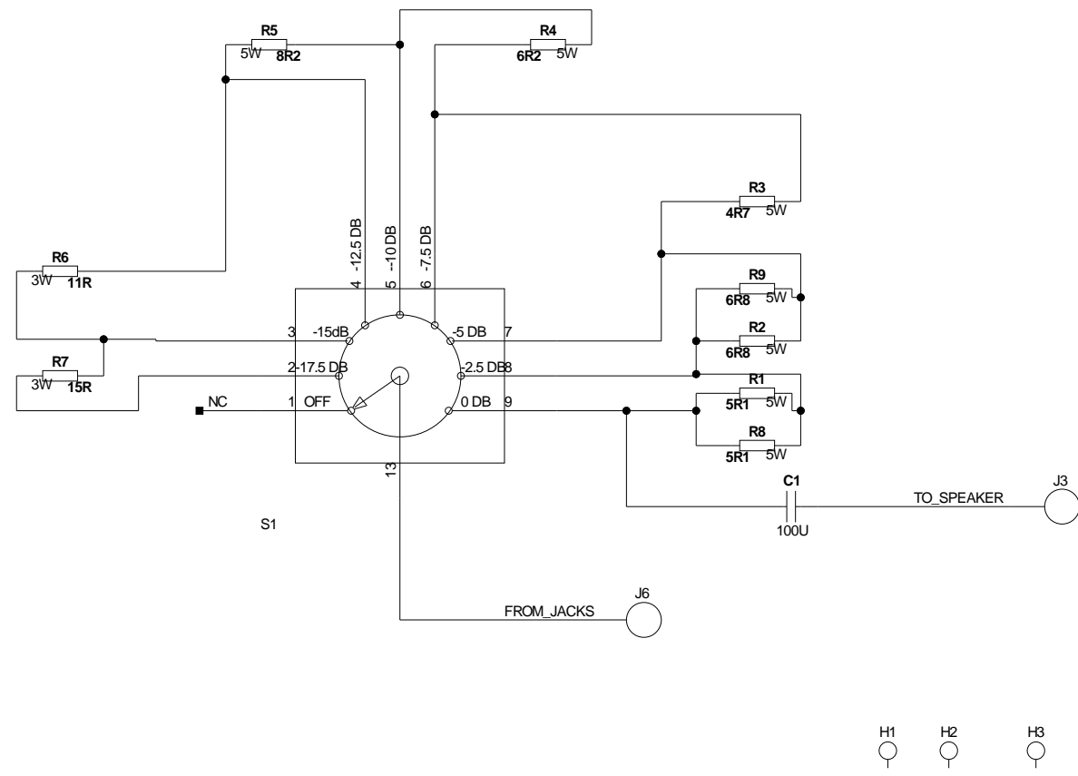
ATTENUATION PCB- SINGLE LAYER
