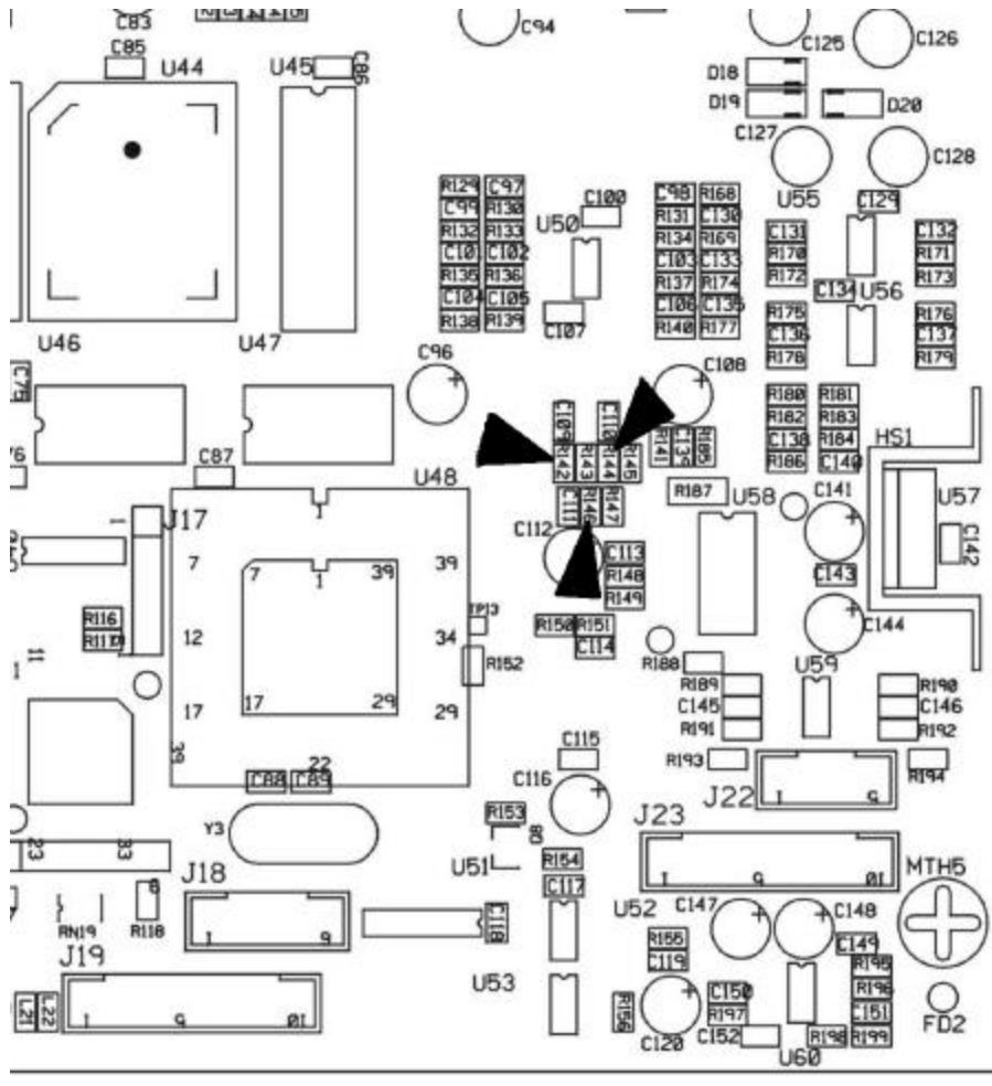
location of R142,R144, R146 on main board PDC0147
