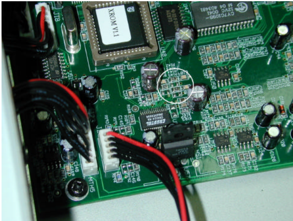
illustration of R142,R144, R146 on main board PDC0147
