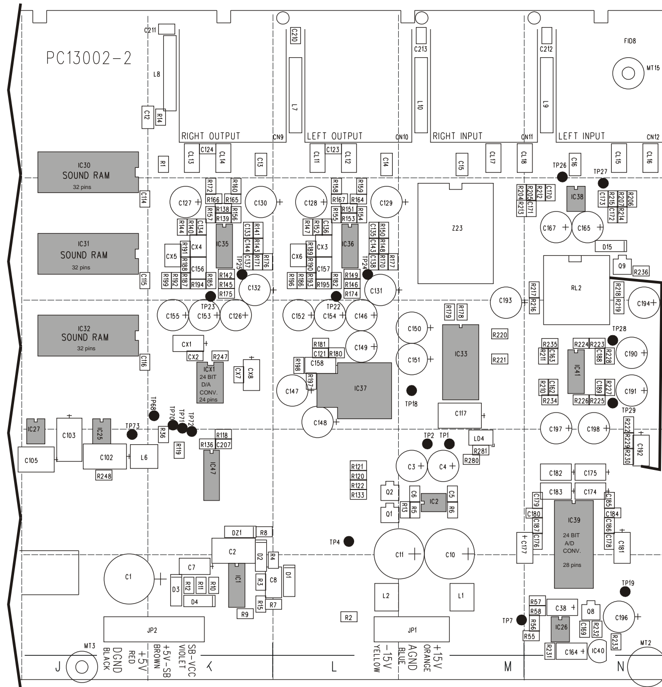
PCB layout, Main Board, PC13002-2, analog section
