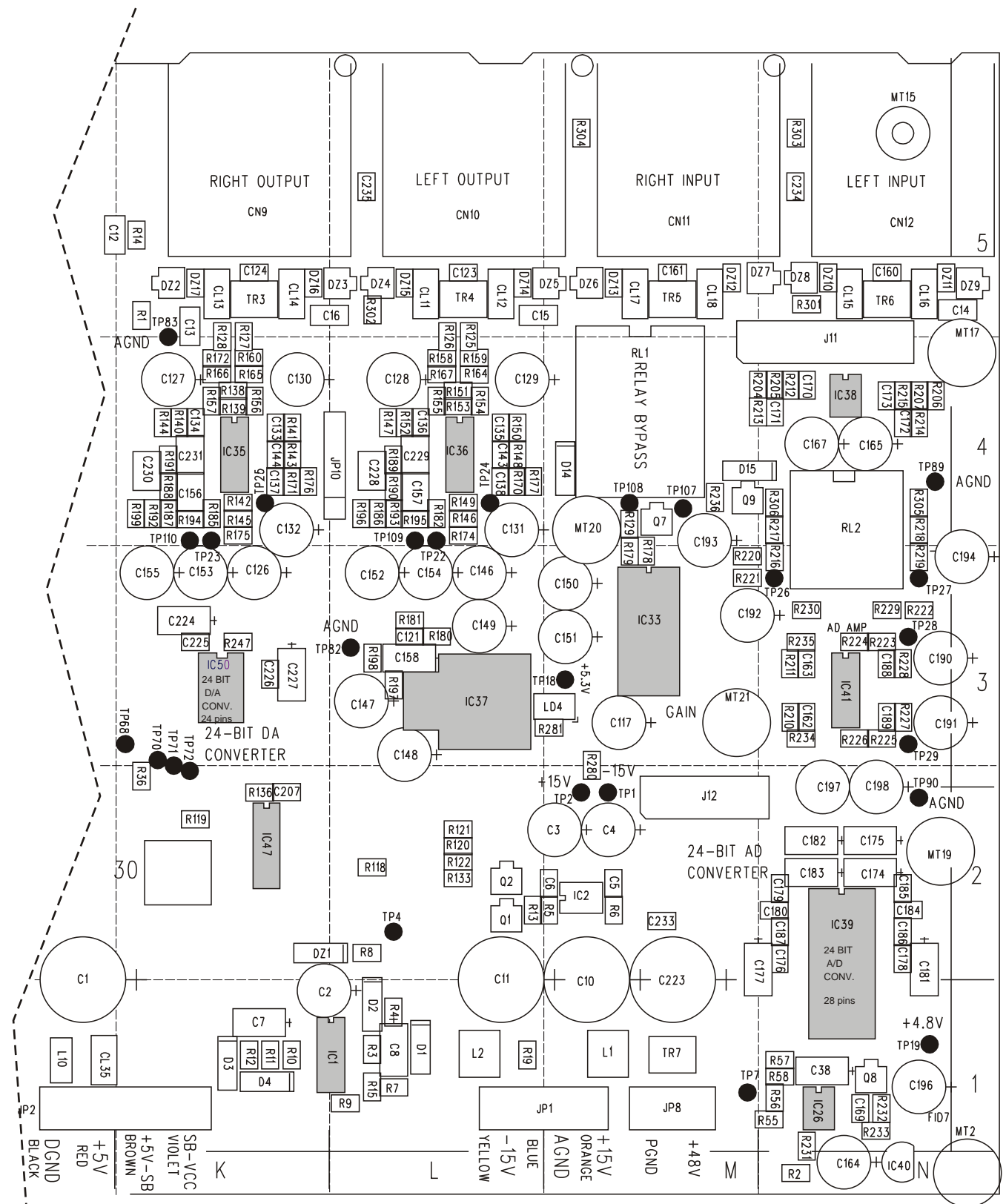
PCB layout, G-Force Main Board, PC13002-4, analog section
