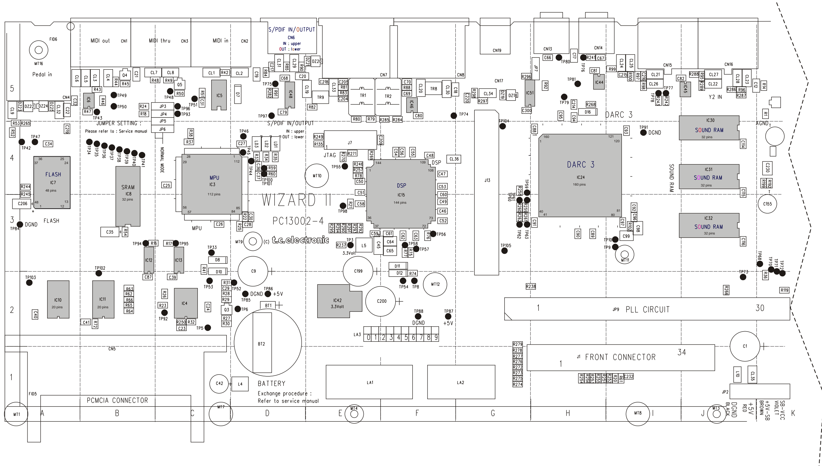
PCB layout, G-Force Main Board, PC13002-4, digital section
