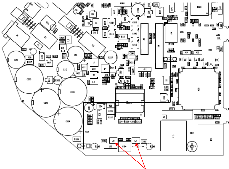
Placement of L7 and L12
