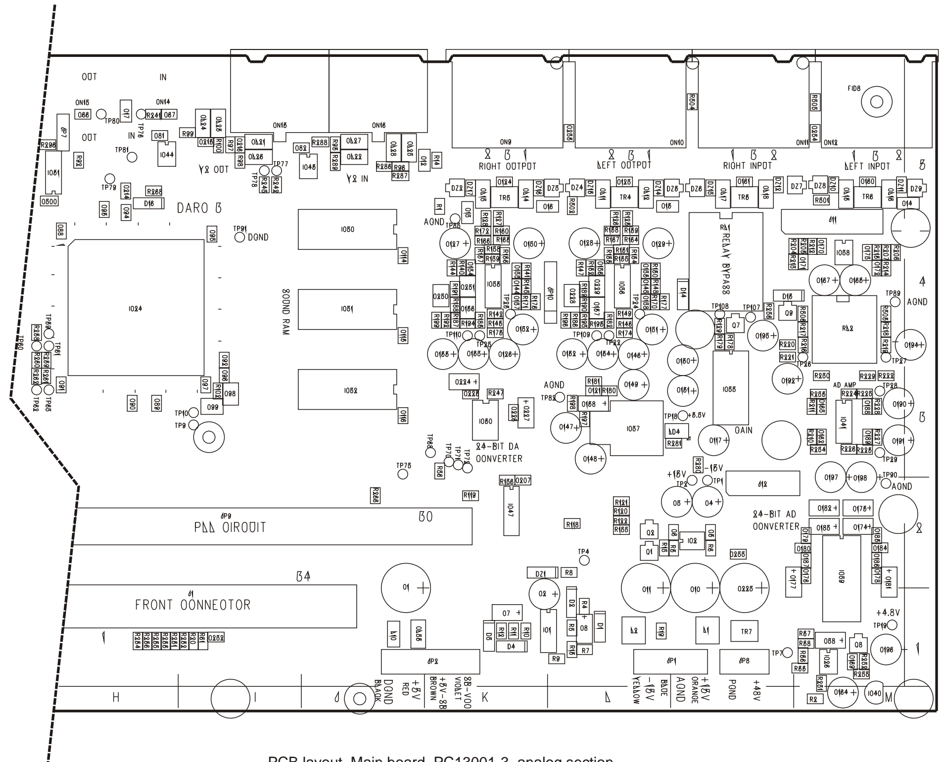
PCB layout, Main board, PC13001-3, analog section
