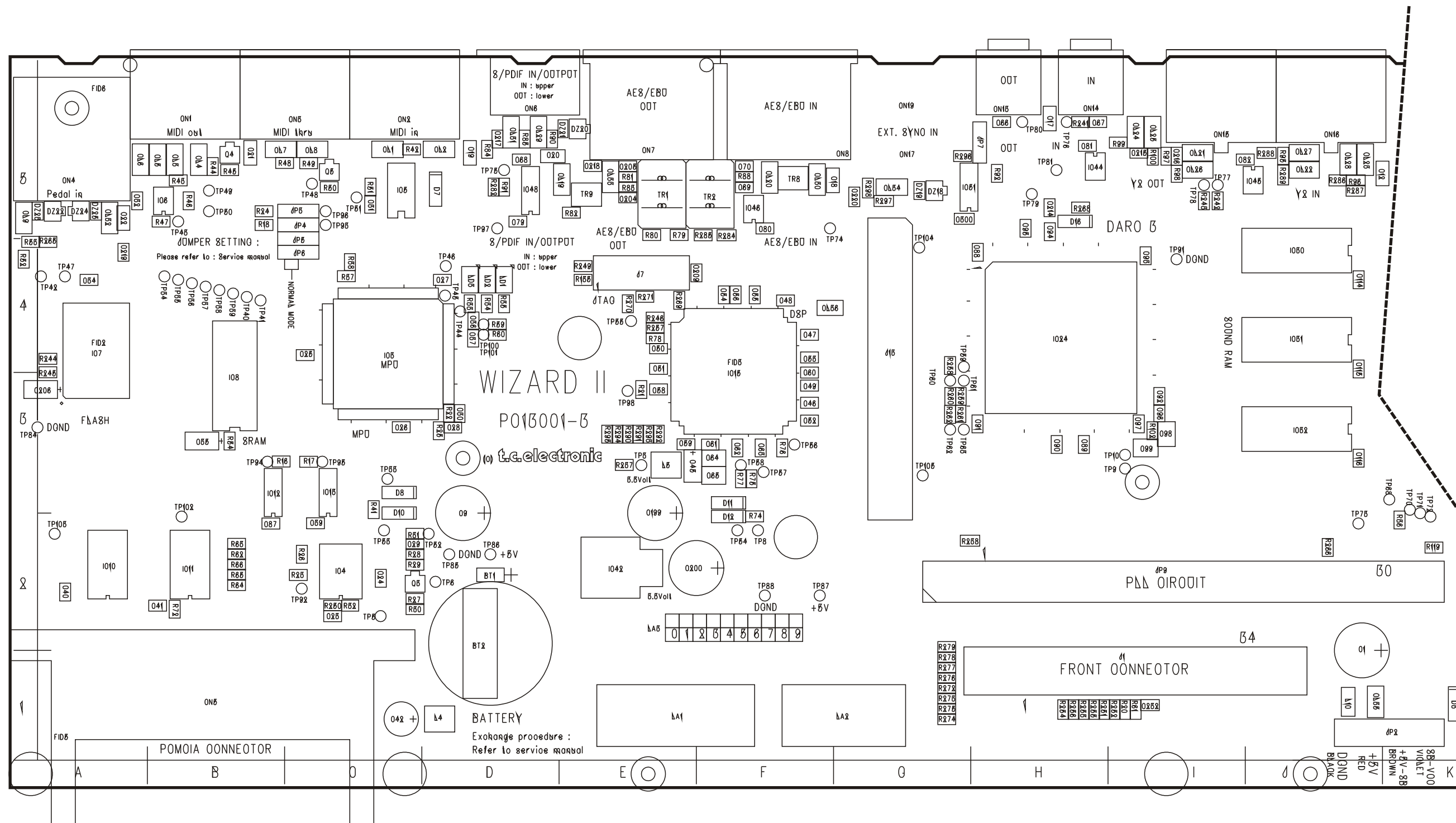
PCB layout, Main board, PC13001-3, digital section
