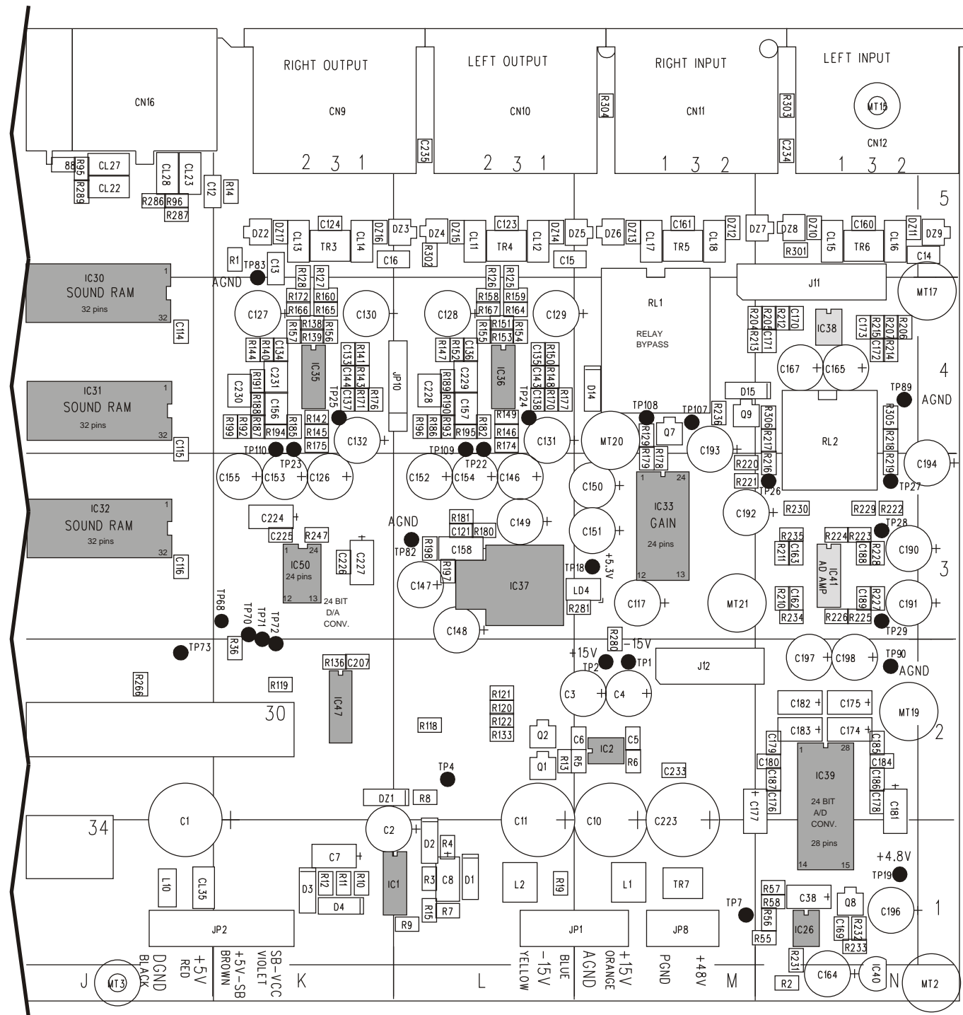
PCB layout, Main Board, PC13001-4, analog section
