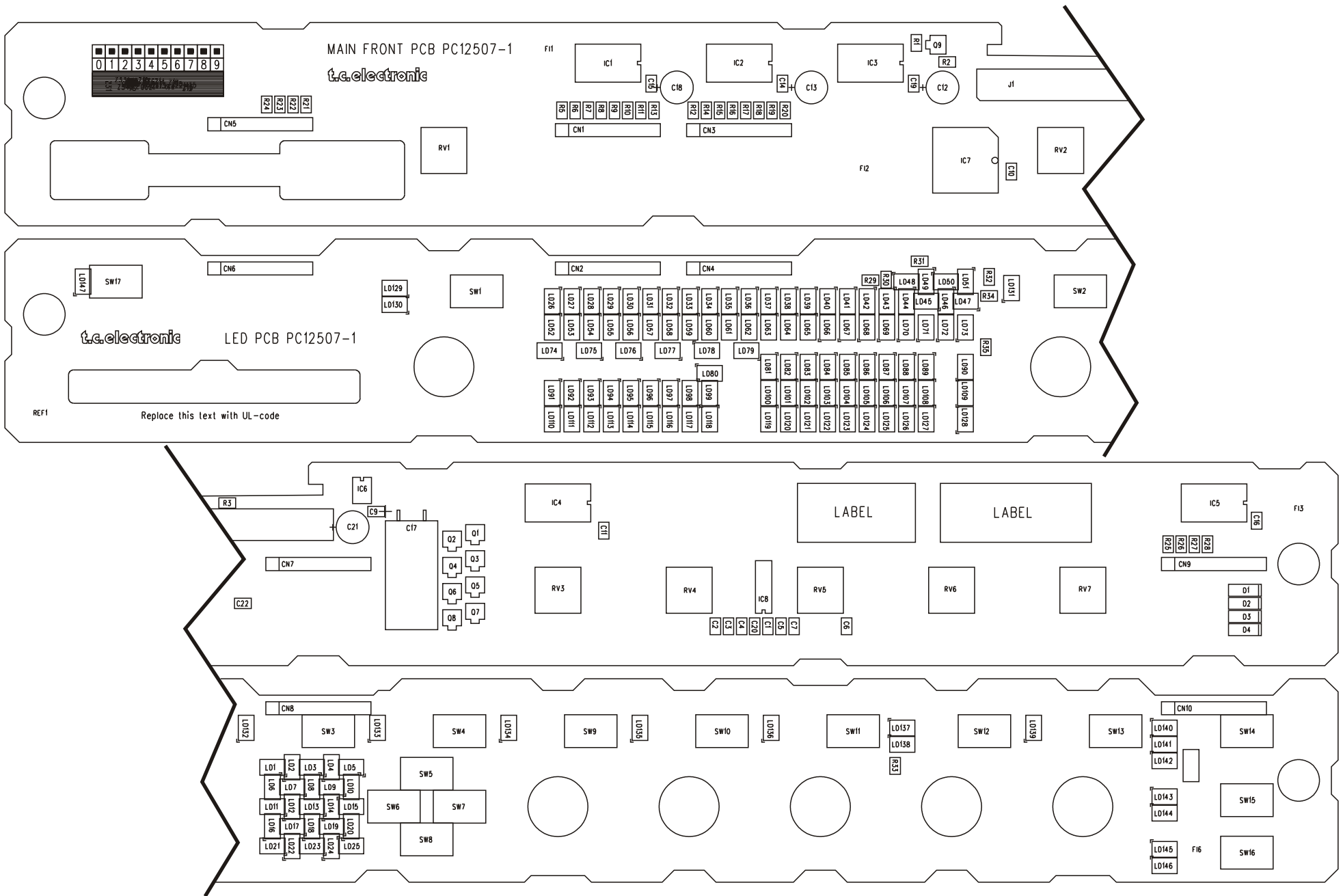
Component layout, Finalizer Express, Front PCB, PC12507-1
