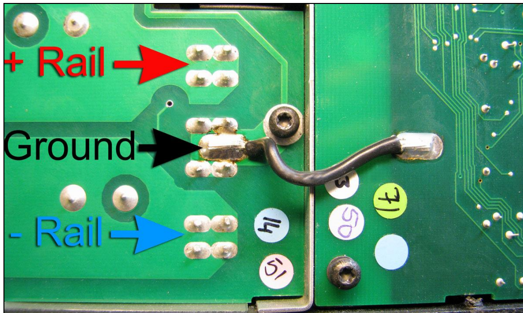
Measuring points
