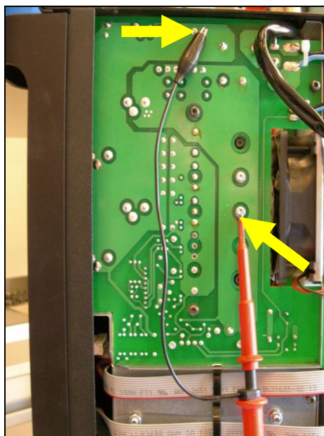
Measuring points for SP130F.
