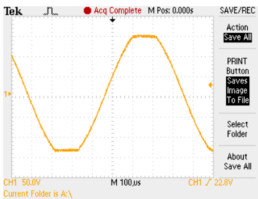
Wave measured at 1.3kHz.
