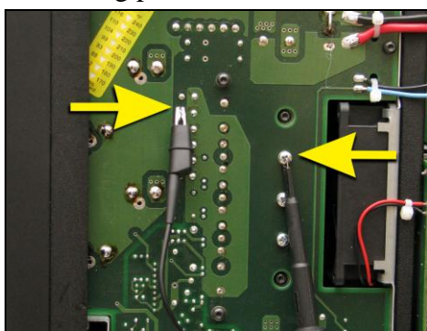
Measuring points for SP140F.
