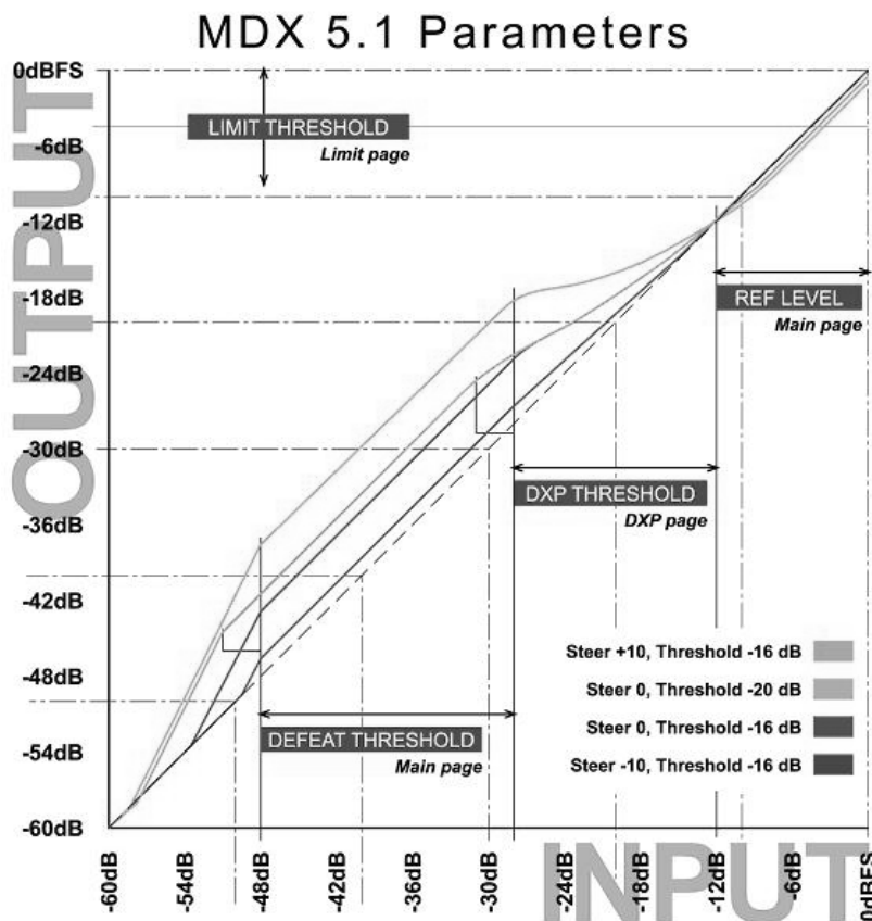
Fig 5. MDX5.1 Level Diagram for different Steer and Threshold settings.. Defeat Threshold relates to DXP Threshold which relates to Ref Level. Limit Threshold only relates to Digital Full Scale output level.
