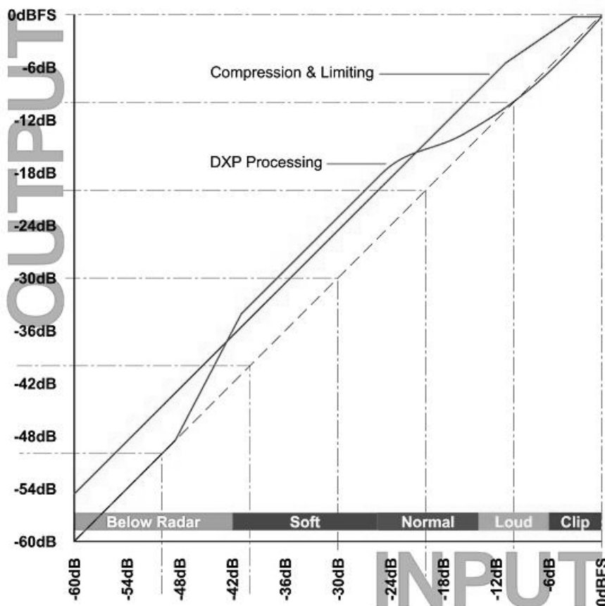
Fig 2. DXP processing vs. traditional Compression and Limiting.
