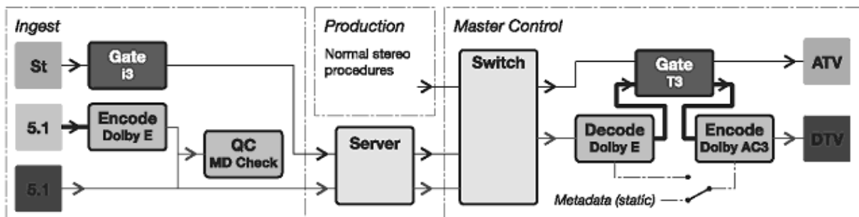
Fig 2. Loudness and Format Control at the station.
